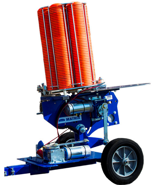
Matrix 6 Wobble - 300 Clay Capacity Shown on optional T-Cart
